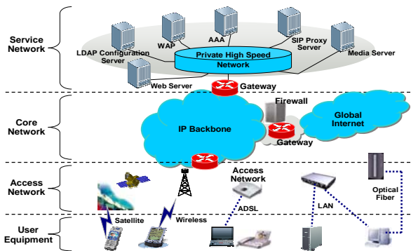
Fig. 1 NGN Network Components
