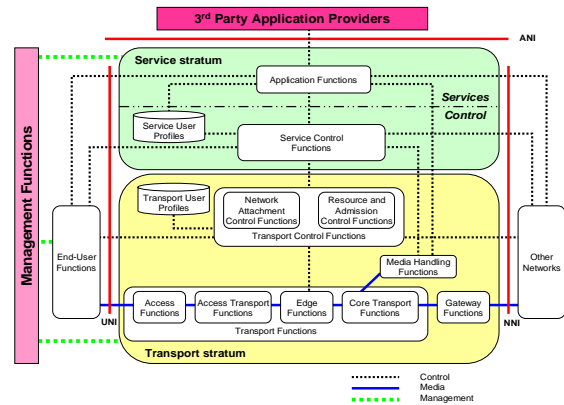
Fig. 2 NGN Functional Architecture
